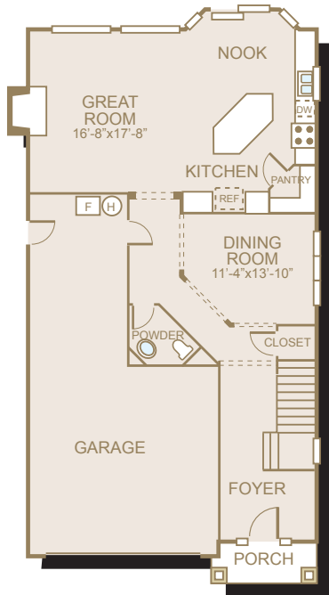
MAIN FLOOR
