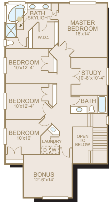
UPPER FLOOR
